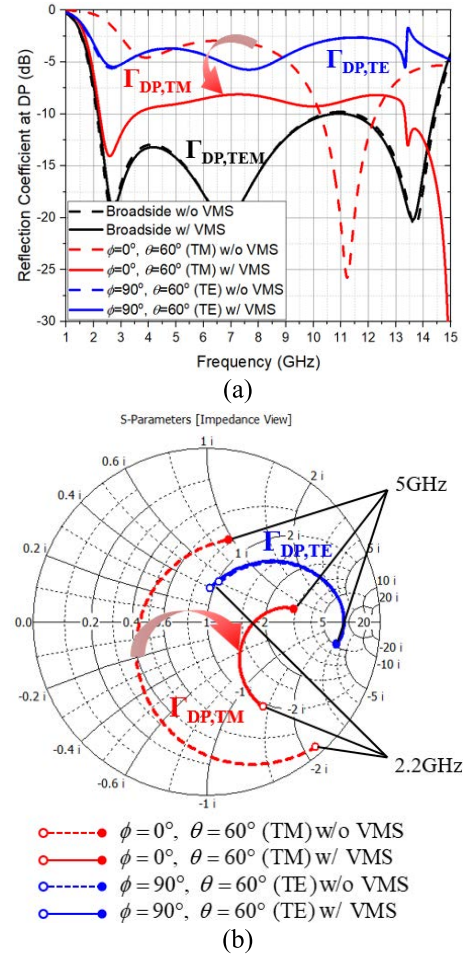
FIGURE 7. (a) Reflection coefficients at the DP of the single-polarized TCDA antenna (Fig. 1(a)) with or without the VMS. When scanning in the plane with \phi = 0^\circ and \phi = 90^\circ , the TM and TE modes are excited, respectively. (b) Curves of the reflection coefficients normalized to 50 \Omega , which are drawn in the Smith chart for 2.2 to 5 GHz.
