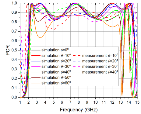
FIGURE 12. Simulated and measured PCRs of the unit cell and fabricated 40 × 40 array structure.
