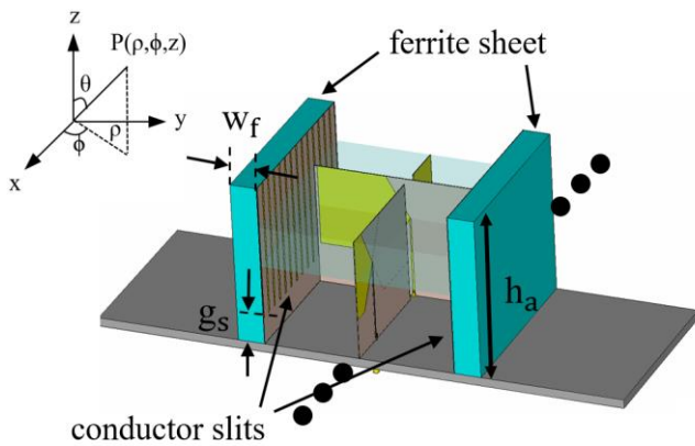
Figure 1. Simulated unit cell of antenna model
