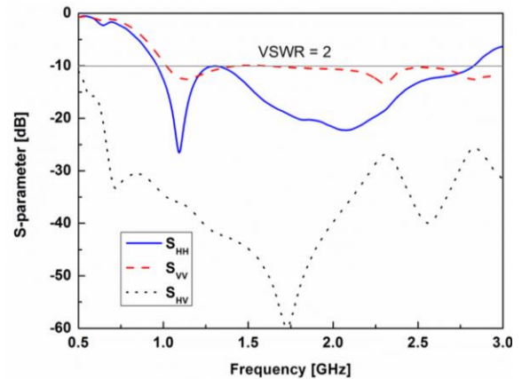
Figure 2. Simulated S-parameter of proposed 1-D TCDA antenna
